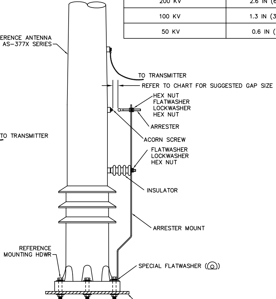
FEEDPOINT 3 CONFIGURATION
