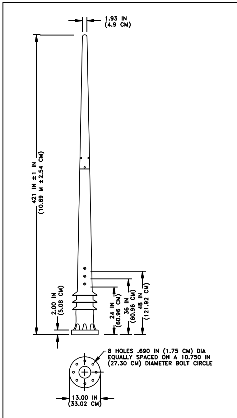
Figure 4-1. Installation Data
